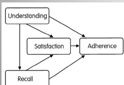
Ley's Model
